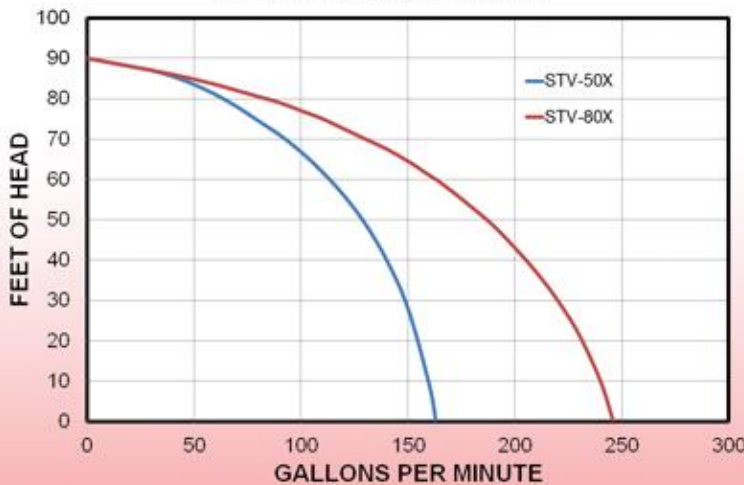
PERFORMANCE CURVES
